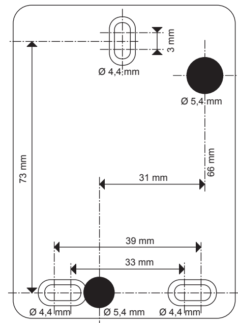
Engineering drawing
